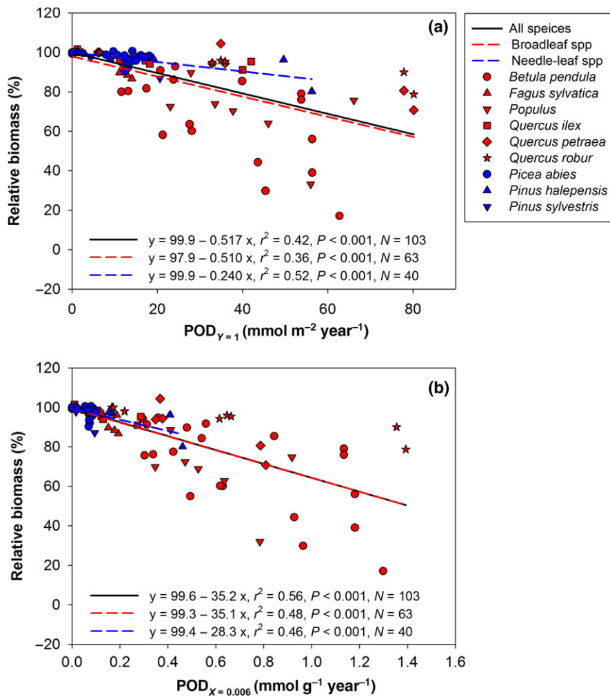
FIGURE 3 Relative biomass of nine European tree species plotted against the annual phytotoxic ozone dose (POD # ; # is a cut-off threshold) expressed per unit leaf (a) area and (b) mass. Relative biomass and POD # data from multiyear experiments are normalized to a single-year basis (see Section 2). The dashed red and blue lines represent the regressions of broadleaf and needle-leaf species, respectively, while the solid black line represents the general relationship across all species
